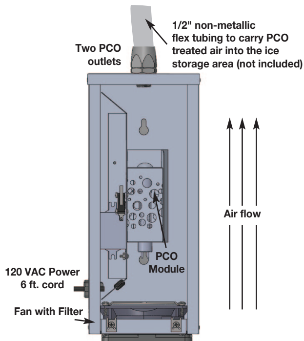
PCO process oxidizes contamination into basic molecules
